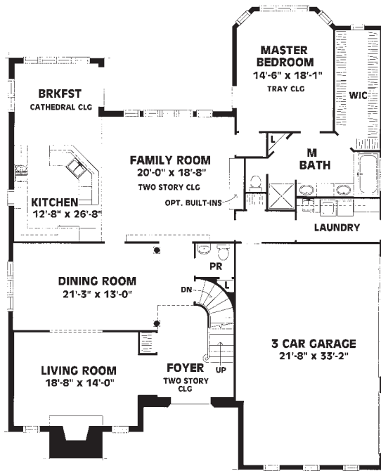
1ST FLOOR PLAN LIVING 2577 S.F. GARAGE 748 S.F.
